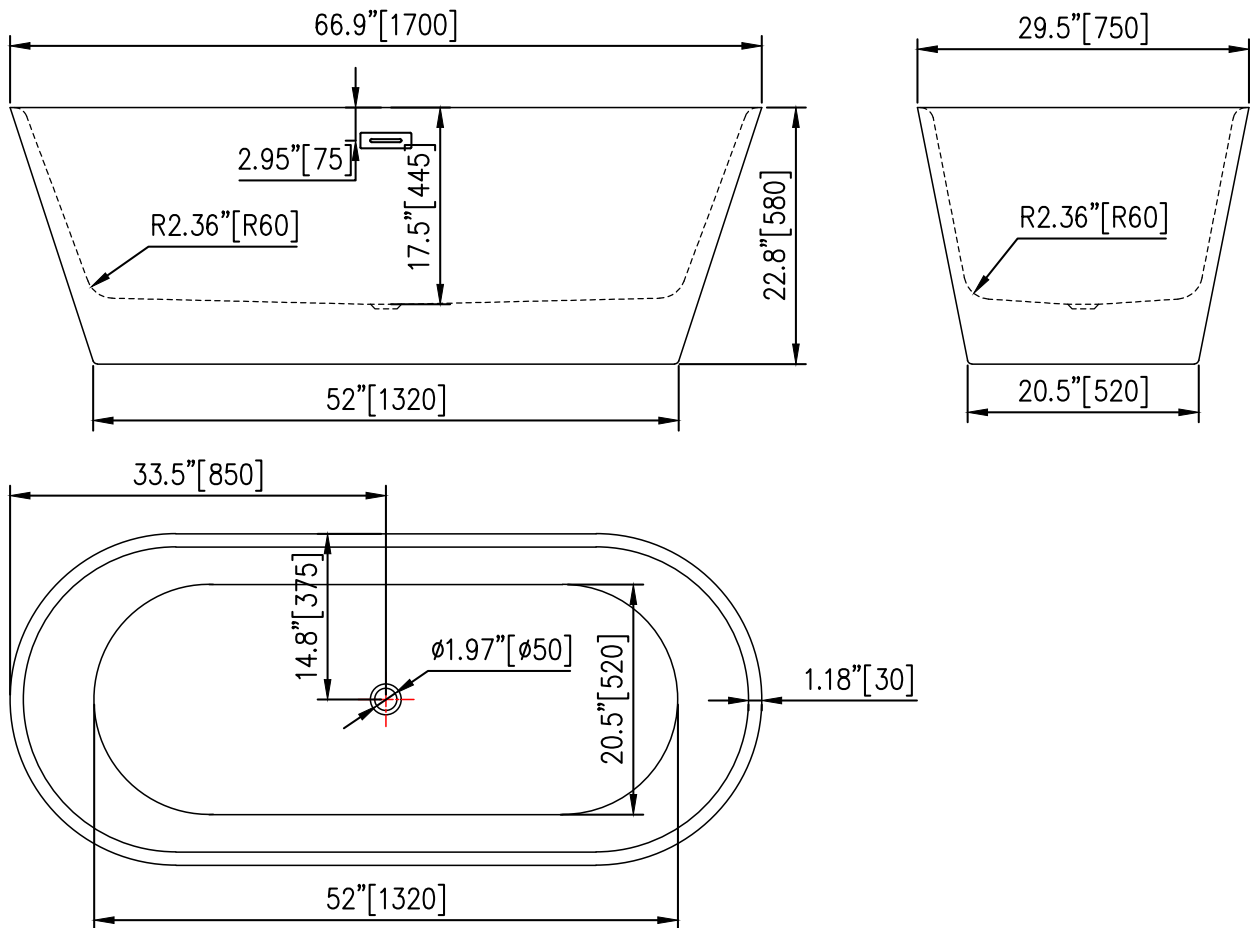
Cut Sheet of the tub
