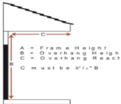
Overhang Requirements
